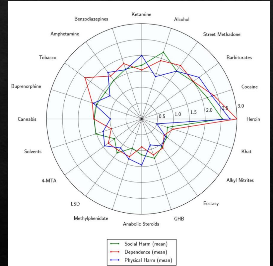
Rational harm assessment of drugs radar plot
