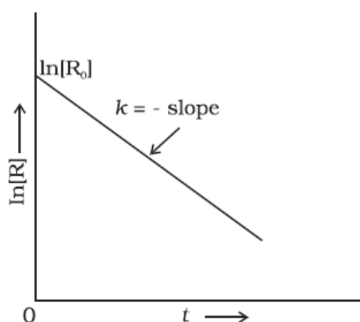
Fig. 2. A plot between \ln [R] and t for a first order reaction.
