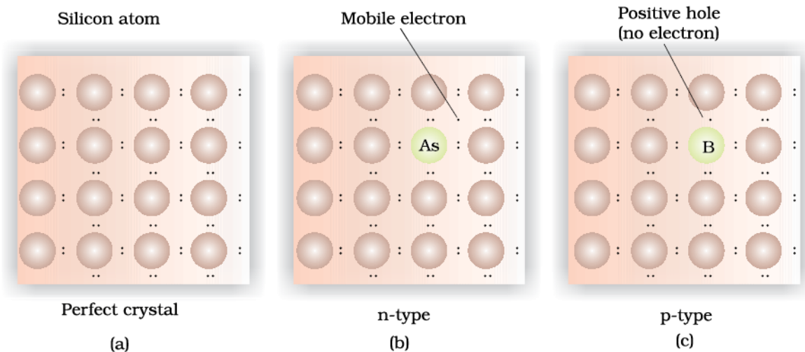
Fig. 2: Creation of n-type and p-type semiconductors by doping groups 13 and 15 elements.
