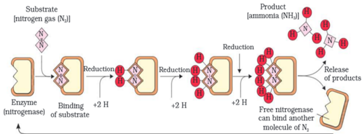
Figure 3: Steps of conversion of atmospheric nitrogen to ammonia by nitrogenase enzyme complex found in nitrogen-fixation bacteria.
