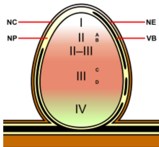
Figure 4: Different zones of an indeterminate root nodule
