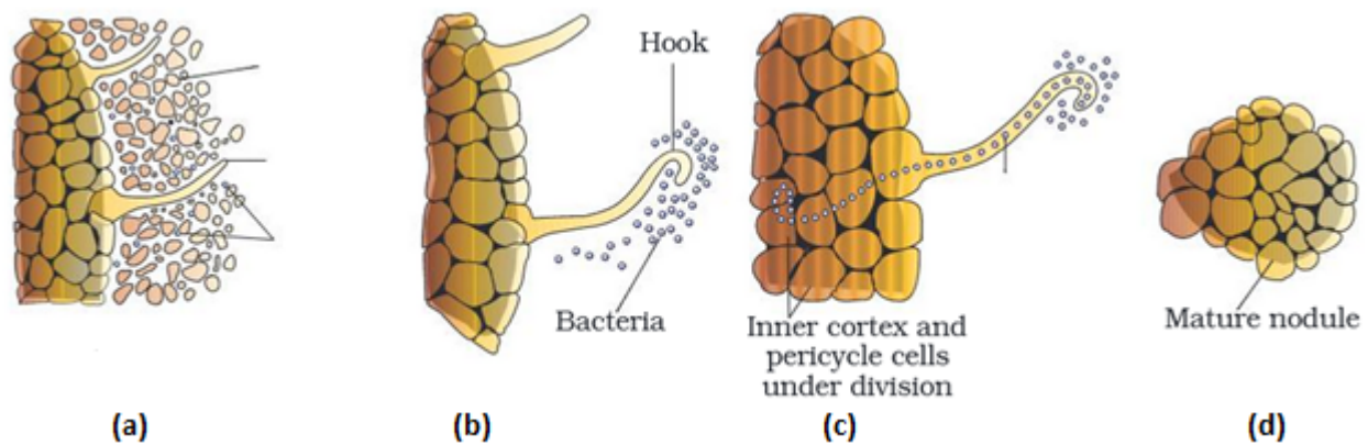
Figure 2: Development of root nodules in soybean: (a) Rhizobium bacteria contact a susceptible root hair, divide near it, (b) Successful infection of the root hair causes it to curl, (c) Infected thread carries the bacteria to the inner cortex. The bacteria get modified into rod-shaped bacteroids and cause inner cortical and pericycle cells to divide. Division and growth of cortical and pericycle cells lead to nodule formation, (d) A mature nodule is complete with vascular tissues continuous with those of the root
