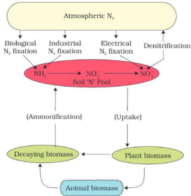
Figure 1: The nitrogen cycle showing relationship between the three main nitrogen pools – atmospheric soil, and biomass
